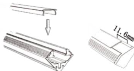
LCB1101A Top Insertion
