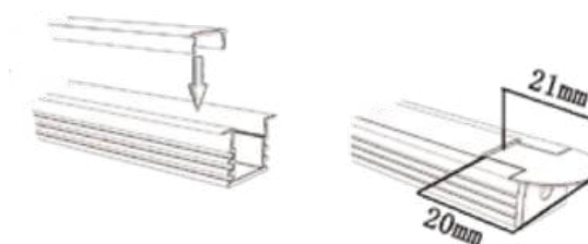
LCB1105A Top Insertion
