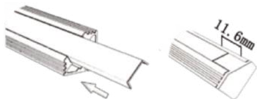
LCB1101 End Insertion
